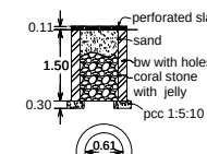
percolation pit
