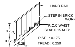
STAIR DETAILS
