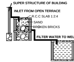
RAINWATER HARVESTING
