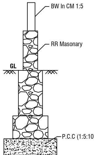
DETAILS OF RR MASONARY
