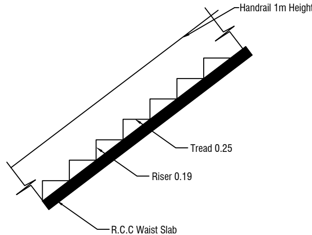
STAIR DETAILS
