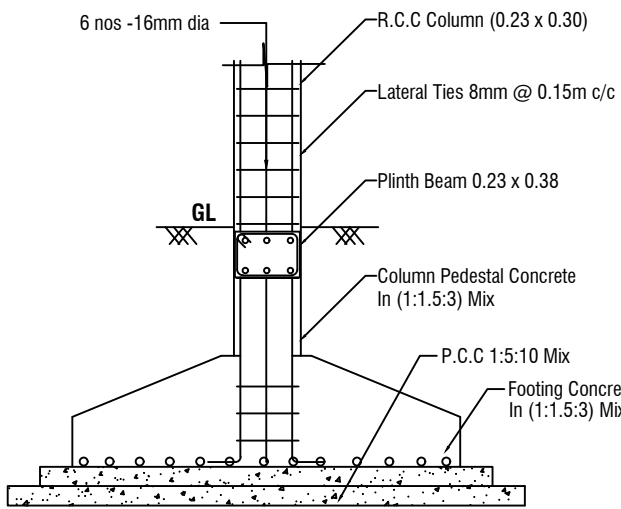
COLUMN FOOTING DETAILS
