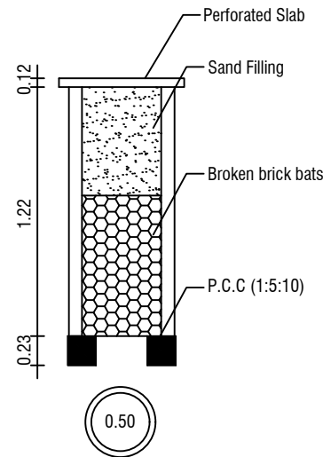
RAIN WATER COLLECTION WELL
