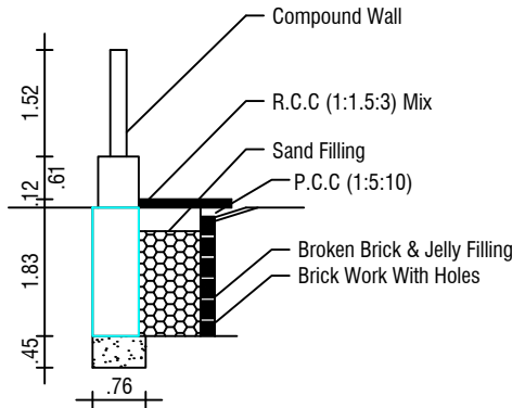
RAIN WATER HARVEST DETAILS
