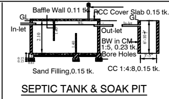
SEPTIC TANK & SOAK PIT
