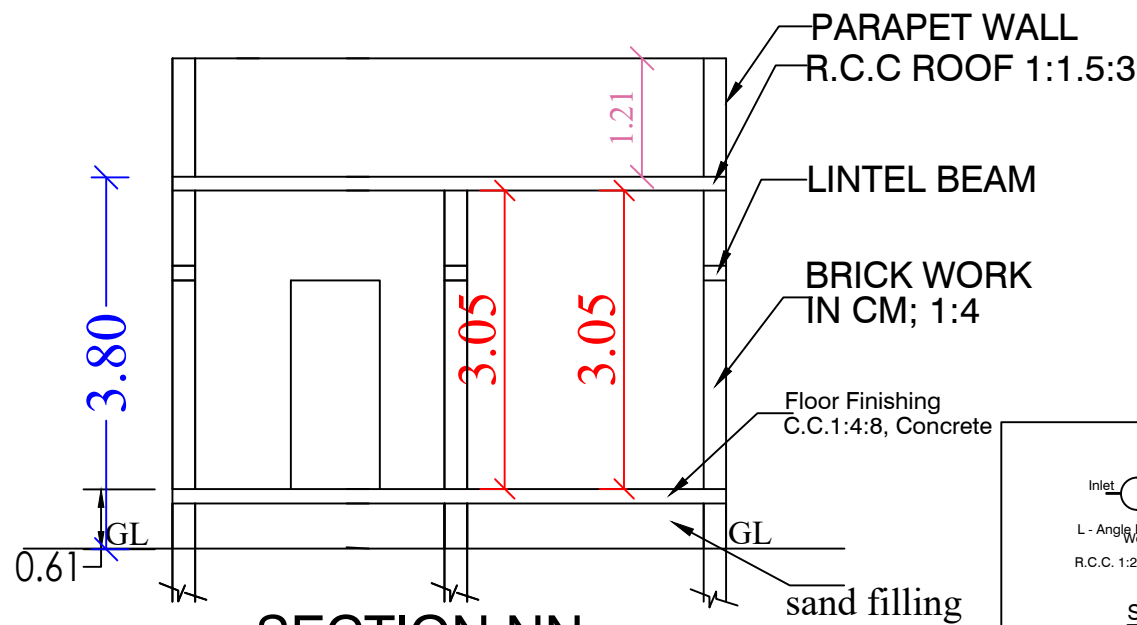
SECTION NN
