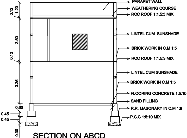
SECTION ON ABCD
