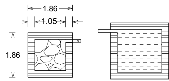
DETAILS OF FILTER BED & WELL
