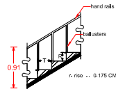
Details of staircase
