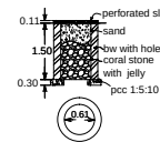
percolation pit
