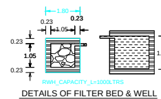
DETAILS OF FILTER BED & WELL
