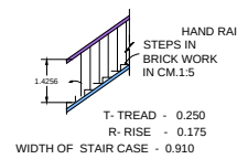
DETAILS OF STAIRCASE
