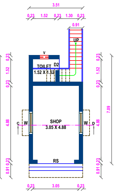
GROUND FLOOR PLAN BLOCK - 02
