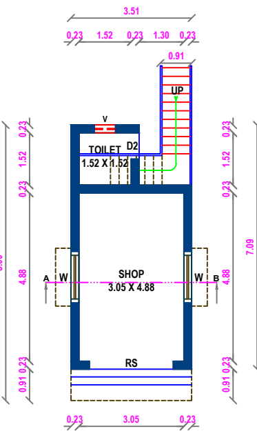
GROUND FLOOR PLAN BLOCK - 01
