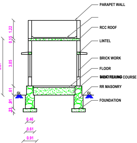
SECTION ON - CD
