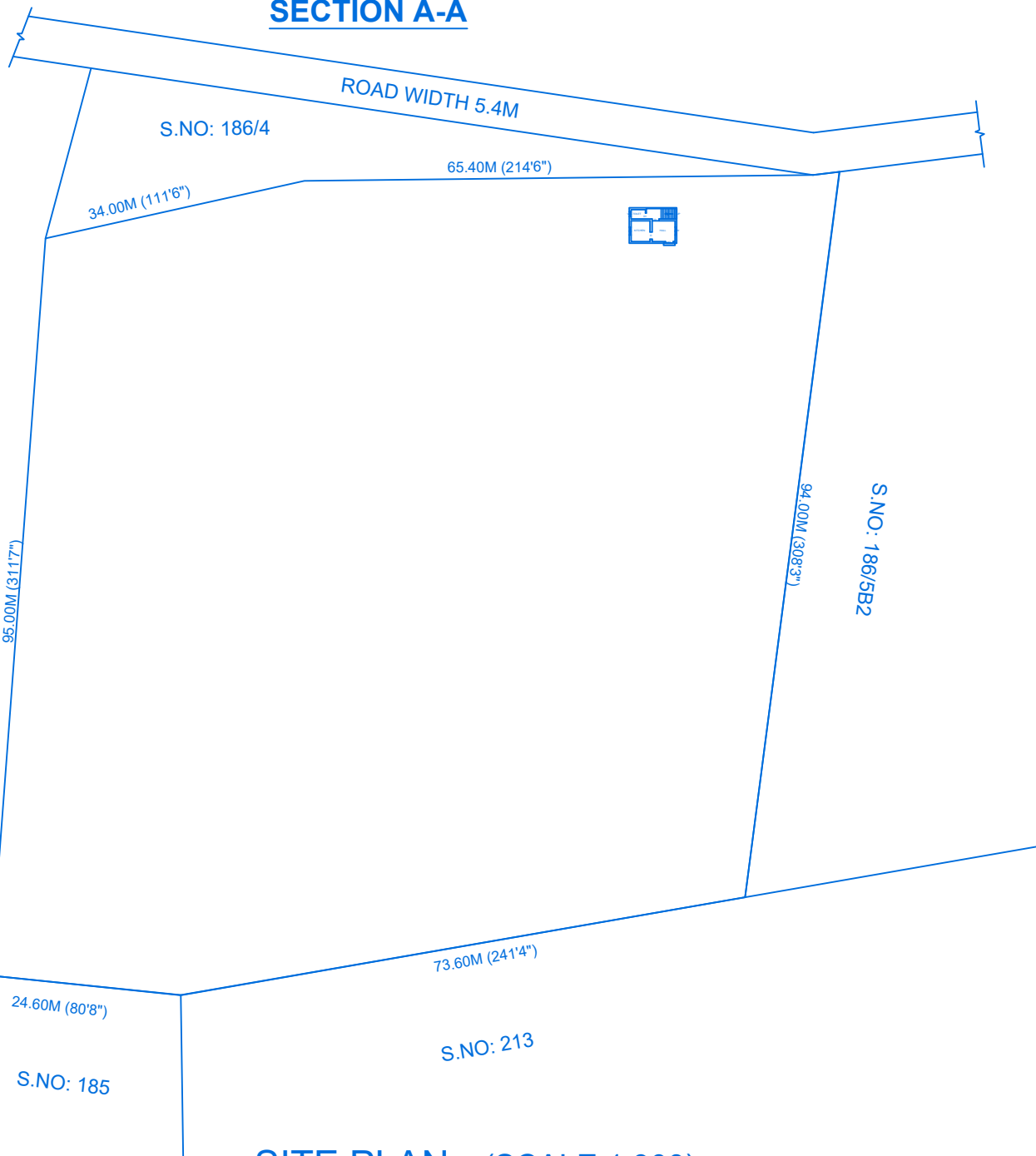
SITE PLAN (SCALE 1:900)
