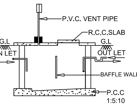
SEC. OF SEPTIC TANK
