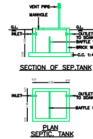
PLAN SEPTIC TANK
