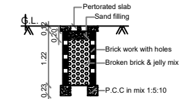
PERCOLATION PIT FOR 30 Sq. m.
