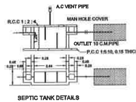
SEPTIC TANK DETAILS
