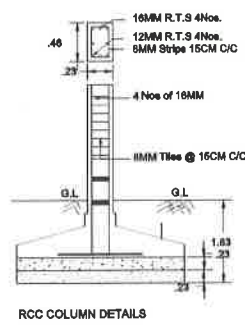
RCC COLUMN DETAILS
