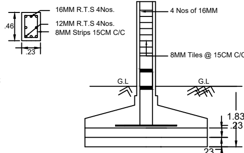
RCC COLUMN DETAILS
