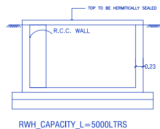
RWH_CAPACITY_L=5000LTRS
