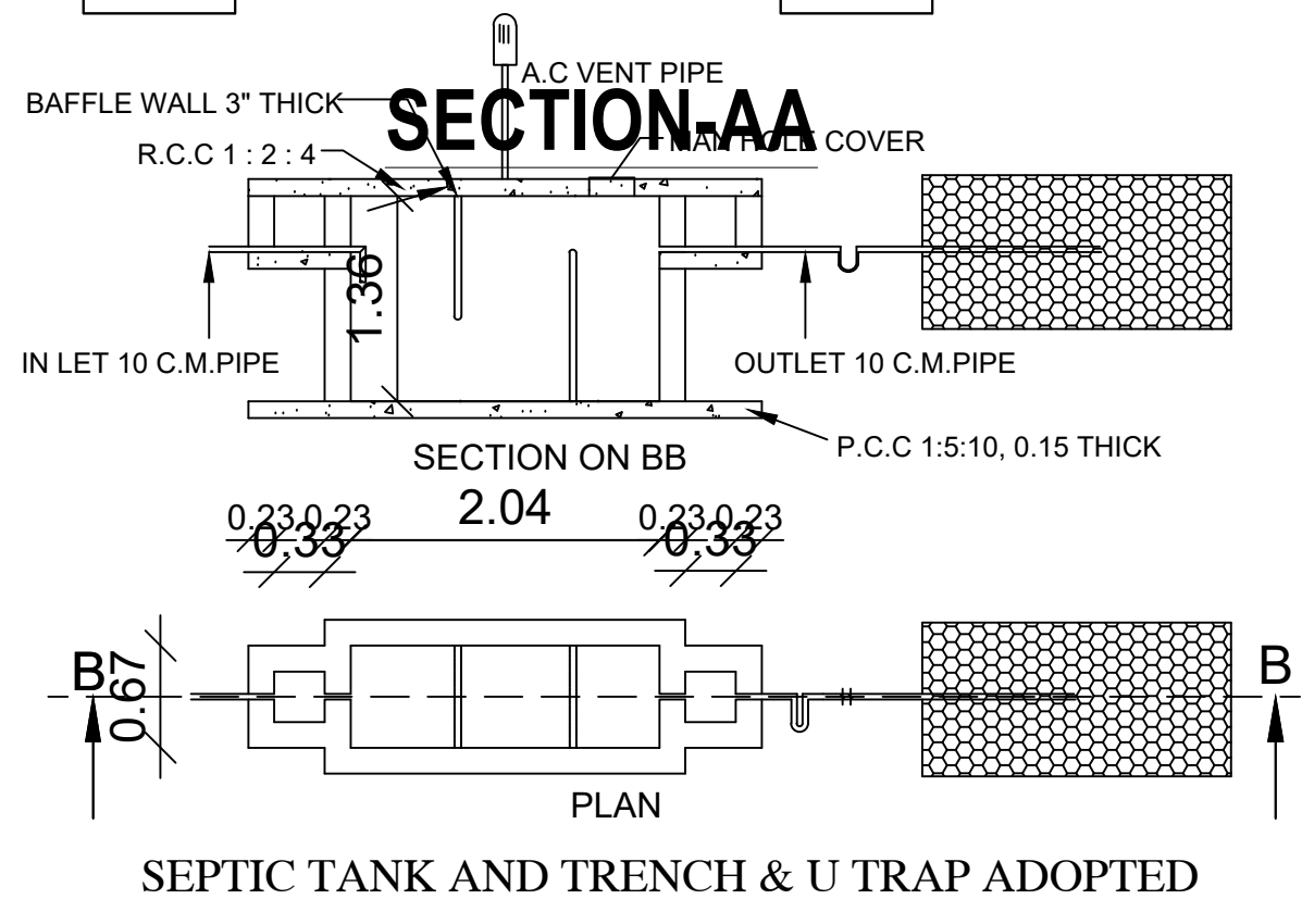
SECTION AA
