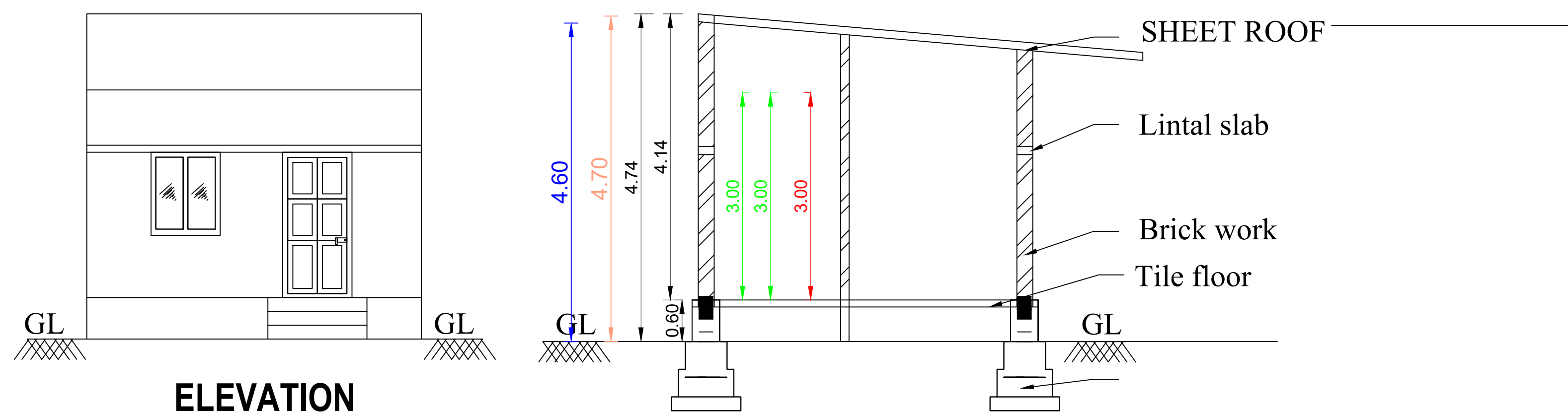
SECTION-AA
