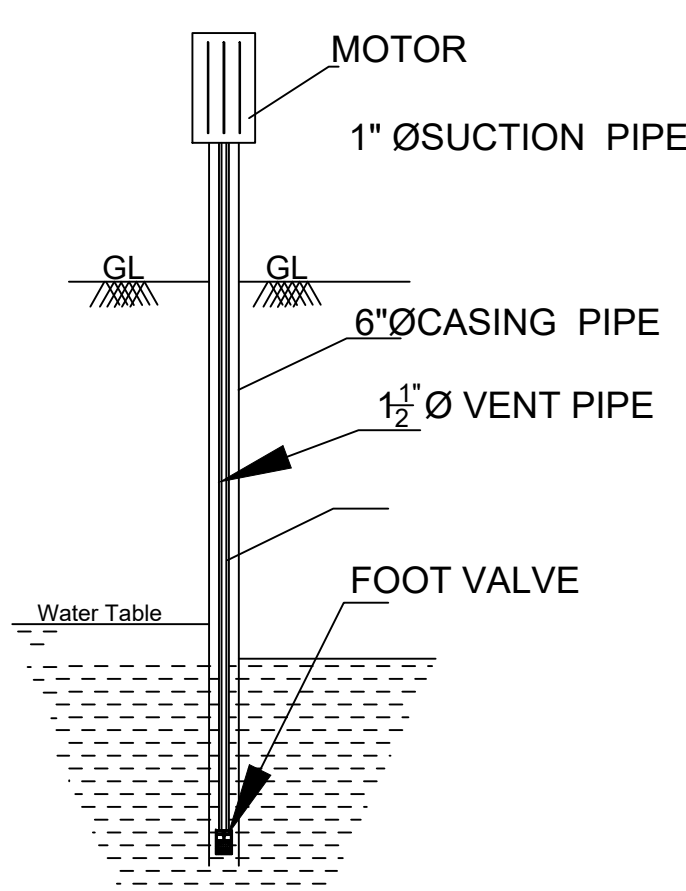
SEC. OF BOREWELL
