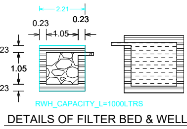
DETAILS OF FILTER BED & WELL
