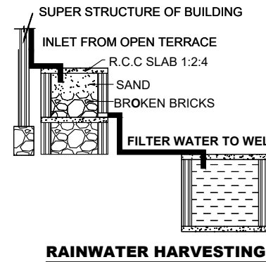
RAINWATER HARVESTING
