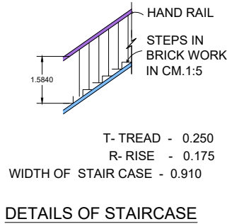
DETAILS OF STAIRCASE
