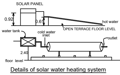
Details of solar water heating system
