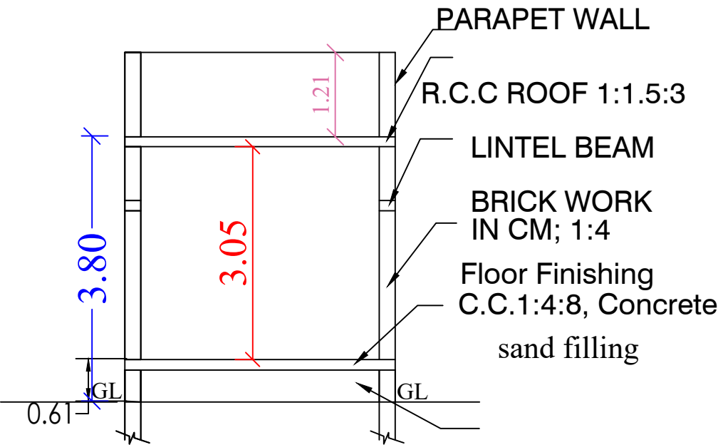
SECTION NN
