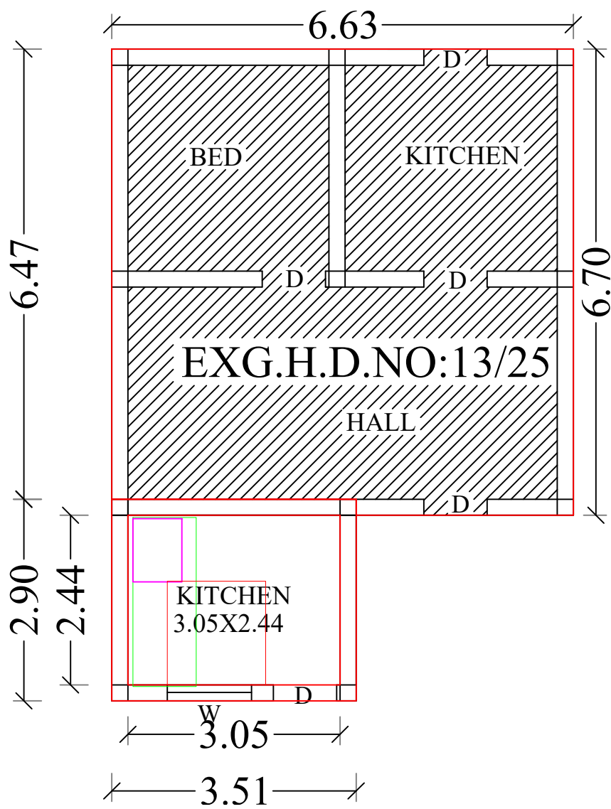
FLOOR PLAN
