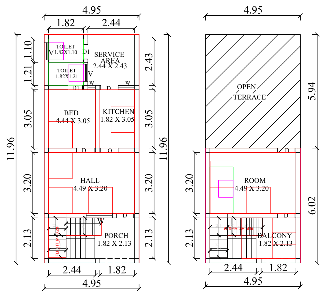
GR PLAN
