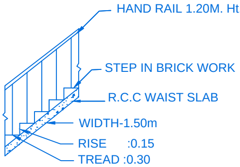
STAIR DETAIL
