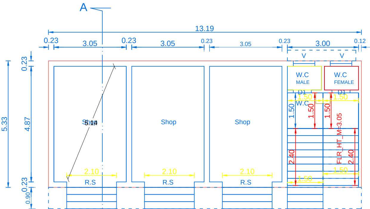
GROUND FLOOR
