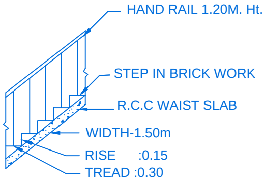
STAIR DETAIL
