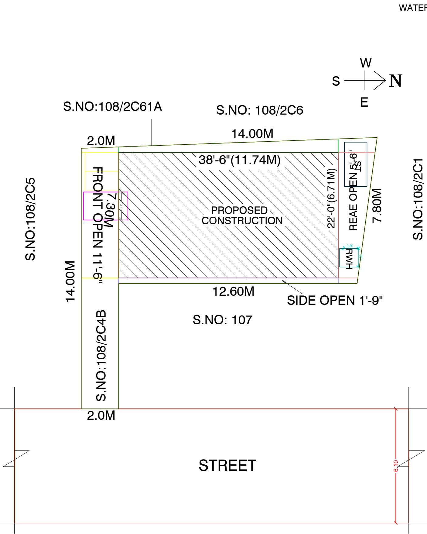
SITE PLAN
