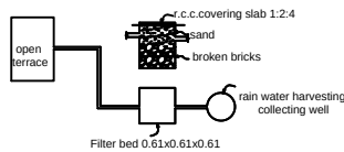
DETAILS OF RAIN WATER HARVESTING SYSTEM
