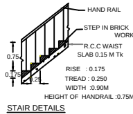
STAIR DETAILS
