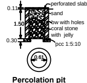
Percolation pit
