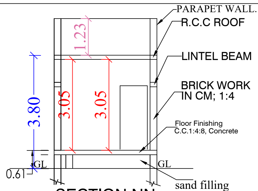
SECTION NN
