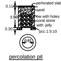
percolation pit
