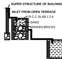
RAINWATER HARVESTING
