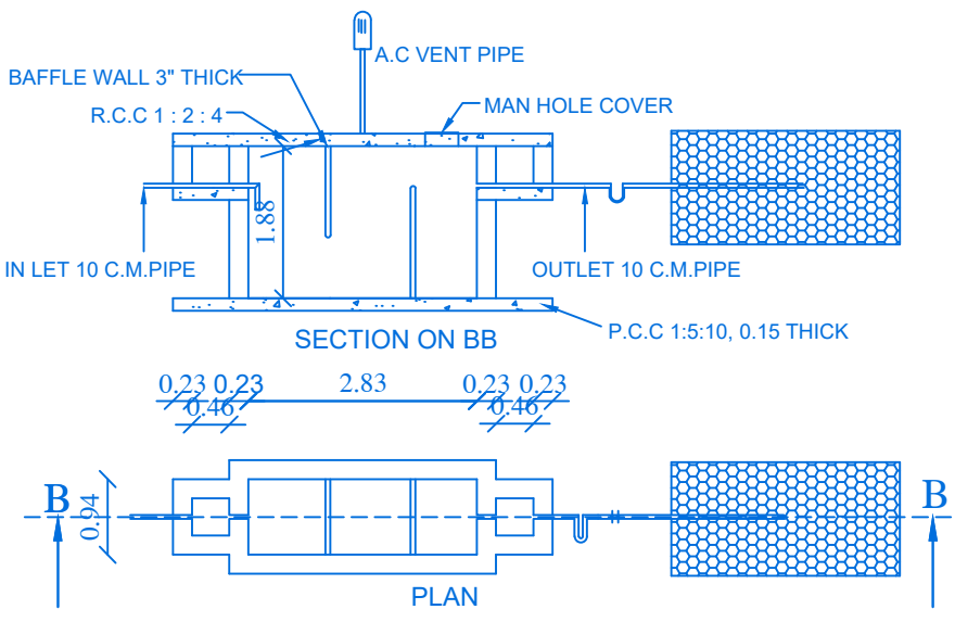
SEPTIC TANK AND TRENCH & U TRAP ADOPTED
