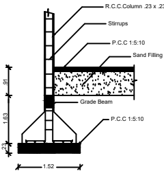
COLUMN DETAIL
