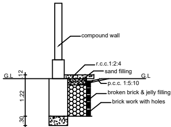
PLINTH BOUNDARY PERCOLATION PIT
