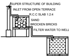
RAINWATER HARVESTING
