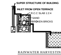
RAINWATER HARVESTING
