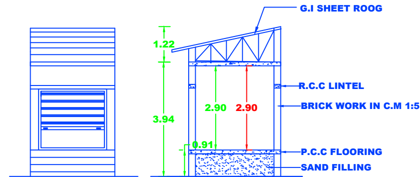
ELEVATION SECTION ON A-A
