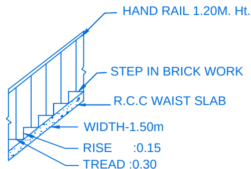
STAIR DETAIL
