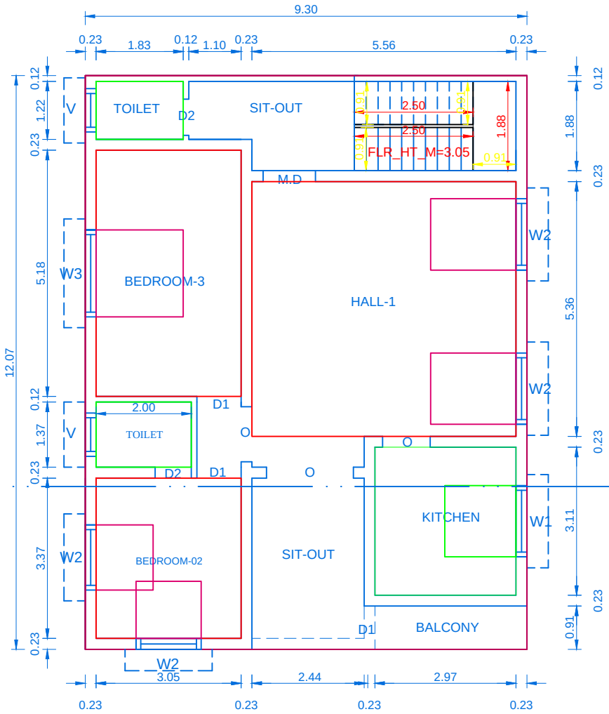
PROP.FIRST FLOOR PLAN
