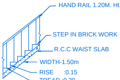
STAIR DETAIL
