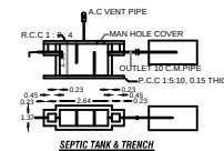
SEPTIC TANK & TRENCH
