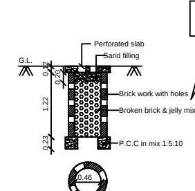
PERCOLATION PIT FOR 30 Sq. m.
