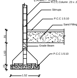
COLUMN DETAIL
