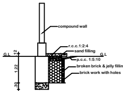
PLINTH BOUNDARY PERCOLATION PIT
