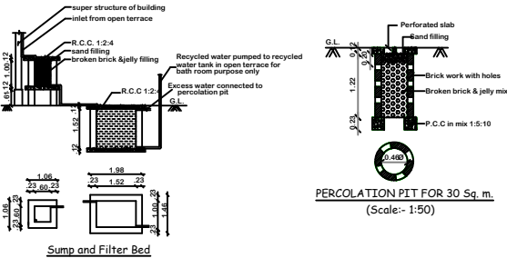
Sump and Filter Bed
