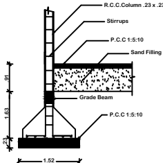
COLUMN DETAIL
