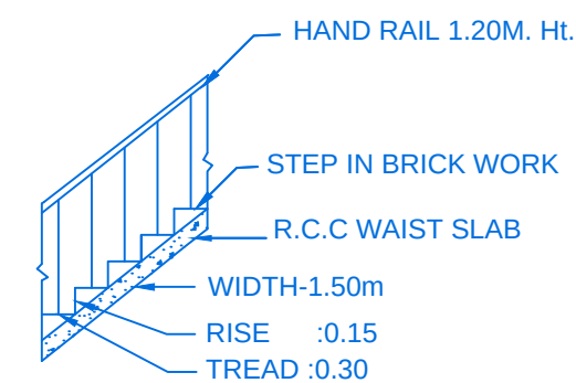
STAIR DETAIL
