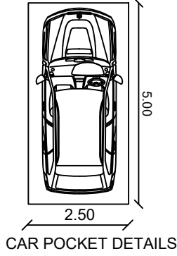
CAR POCKET DETAILS
