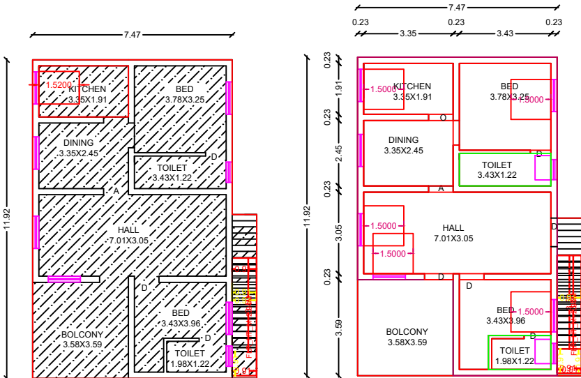
GROUND EXG FLOOR PLAN
