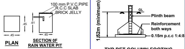
PLAN SECTION OF RAIN WATER PIT TYP.DET.COLUMN FOOTING
