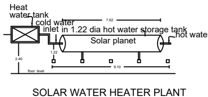
SOLAR WATER HEATER PLANT
