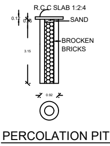
PERCOLATION PIT
