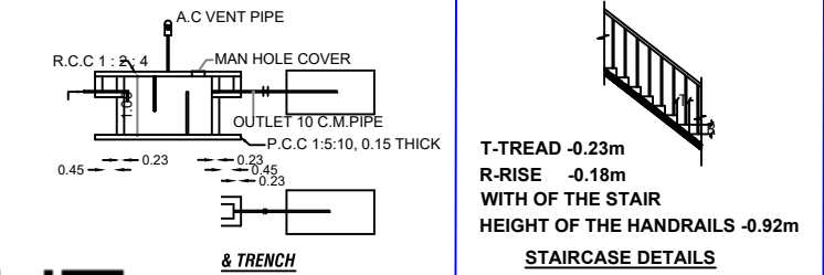
T-TREAD -0.23m R-RISE -0.18m WITH OF THE HANDRAILS -0.92m STAIRCASE DETAILS
