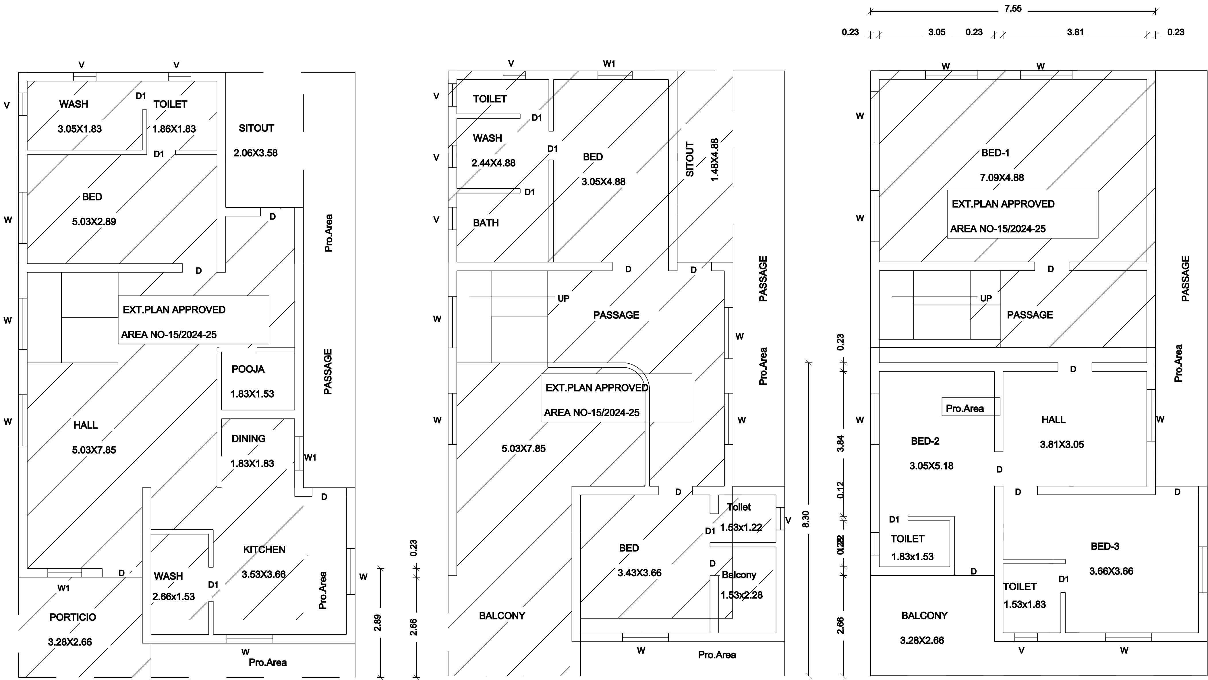
EXT&PRO.S.FLOOR PLAN
