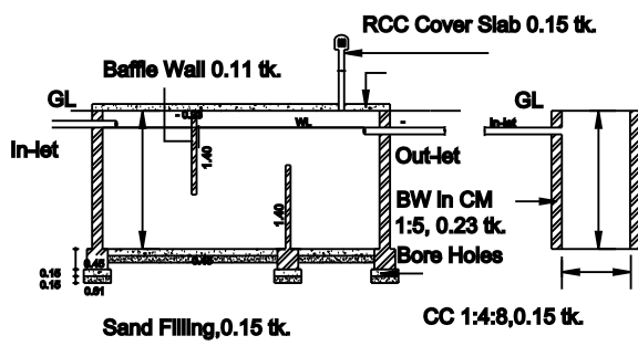
SEPTIC TANK & SOAK PIT (NOT TO SCALE)
