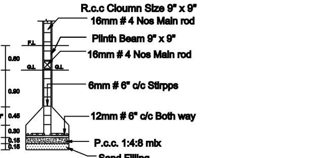
COLUMN DETAIL
