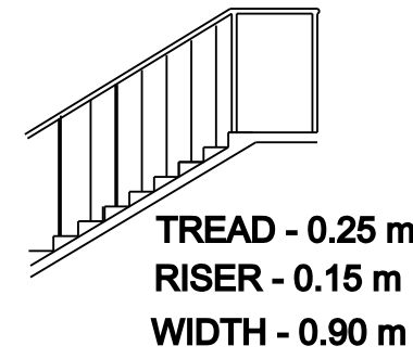
STAIRCASE DETAILS
