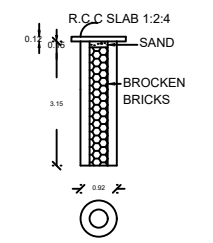
PERCOLATION PIT
