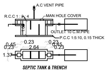
SEPTIC TANK & TRENCH
