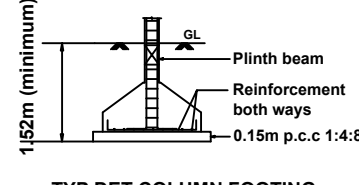
TYP.DET.COLUMN FOOTING
