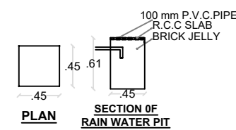
SECTION OF RAIN WATER PIT
