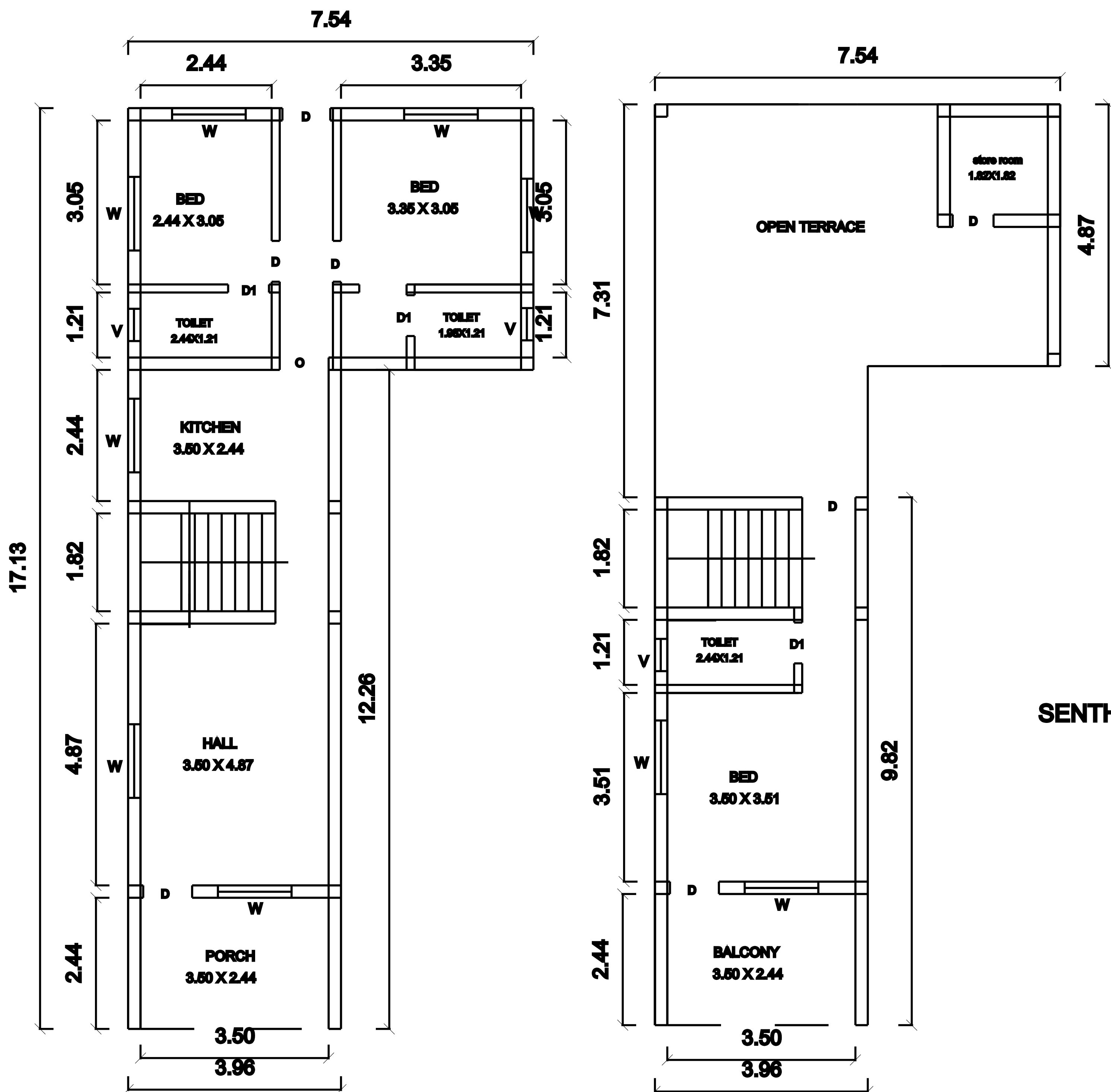
PRO.GROUND FLOOR PLAN
