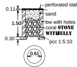
percolation pit
