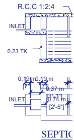
SEPTIC
