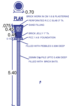
PERCOLATION PIT
