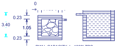
DETAILS OF FILTER BED & WELL
