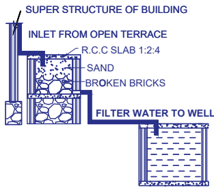
RAINWATER HARVESTING
