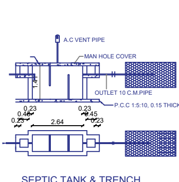
SEPTIC TANK & TRENCH
