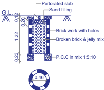
PERCOLATION PIT FOR 30 Sq. m.
