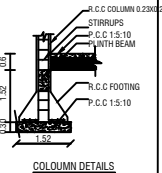
COLUMN DETAILS
