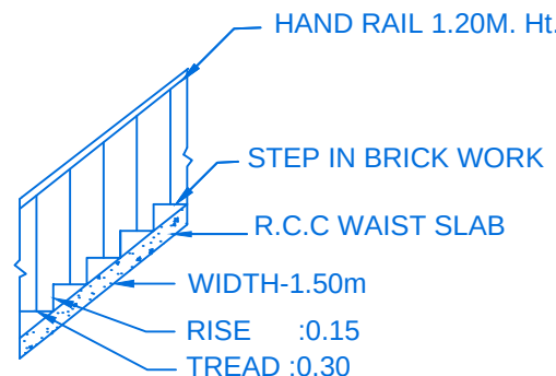
STAIR DETAIL
