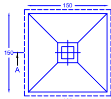
RCC FOUNDATION PLAN (SCALE 1:20)
