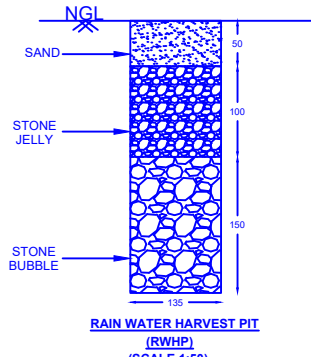
RAIN WATER HARVEST PIT (RWHP) (SCALE 1:20)
