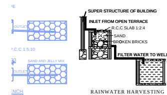
RAINWATER HARVESTING
