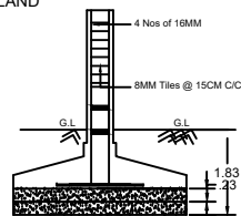
RCC COLUMN DETAILS
