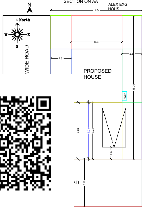
SITE PLAN
